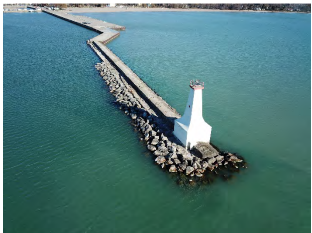
Figure 3.2 Sample photos of GRCA shoreline captured with the UAV. From top left to bottom right; Newcastle, Bond Head Bluffs, Port Hope West Beach and Jetty, Cobourg East Breakwater
